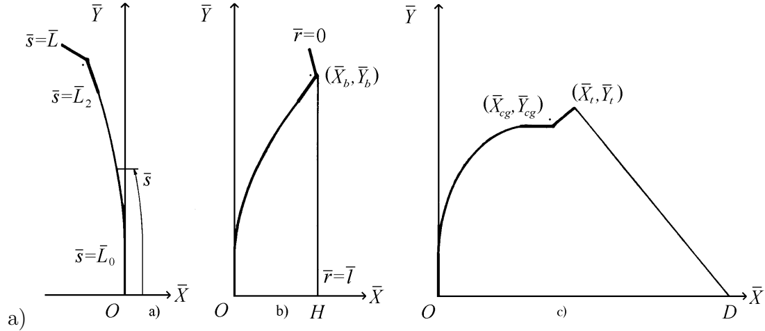
Figure 2: Three situations of the static-recurve bow: a) unbraced, b) braced, c) fully drawn.
