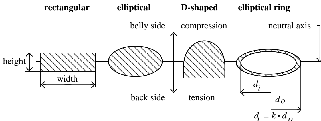
Figure 6: Different shapes of the cross-section of the bow.
