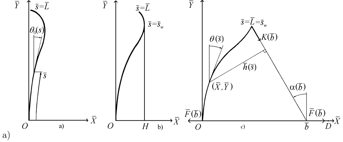
Figure 3: Three situations of the working-recurve bow: a) unbraced, b) braced, c) partly drawn.
