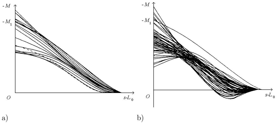
Figure 5: Distribution of the bending moment along the limb of the WR-bow (a) before arrow exit t \leq t_l and (b) after arrow exit t \geq t_l . The broken line represents the distribution along the limb in the static braced situation. The bending moment M_1(s - L_0) in the fully drawn bow is also shown in both figures.
